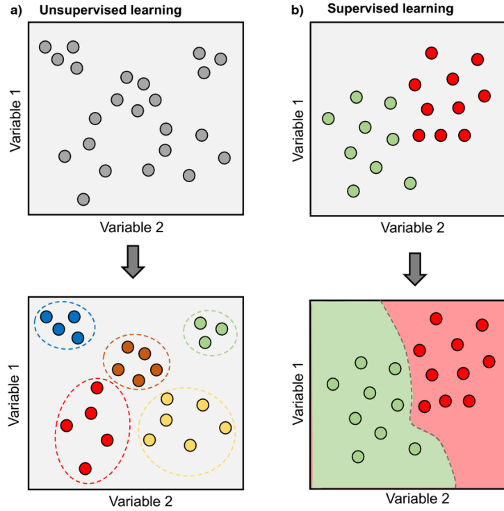
Figure 2.2: Conceptual illustration of unsupervised (a) and supervised (b) learning. Unsupervised methods such as clustering group data based on similarity without labels, while supervised methods such as classification learn decision boundaries from labelled data. Reproduced from [10]
