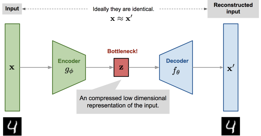
Figure 2.3: An illustration of autoencoders' general architecture and reconstruction task. Reproduced from [12]
