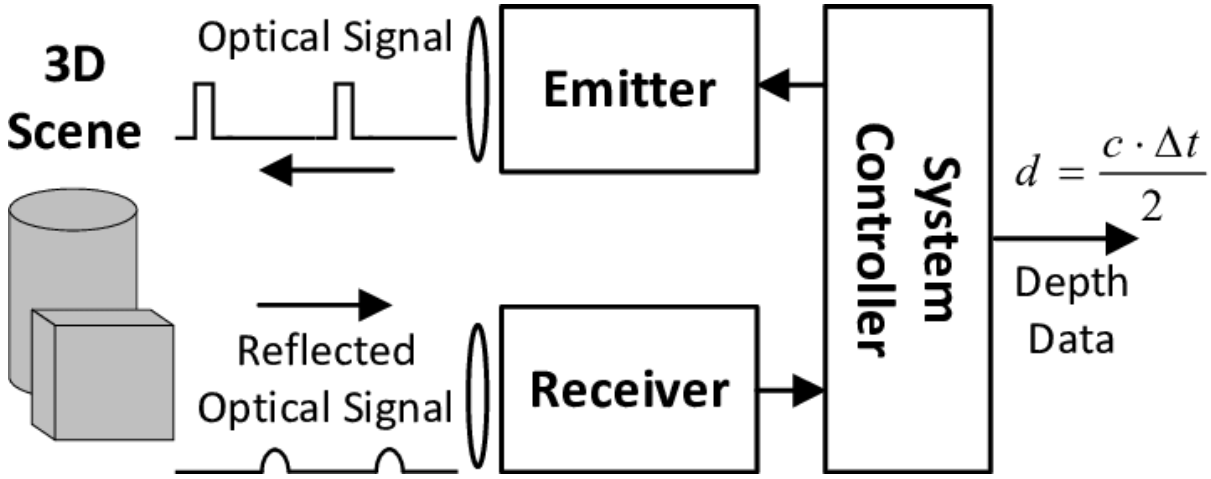
Figure 2.4: An illustration of lidar sensors’ working principle. Reproduced from [16]
