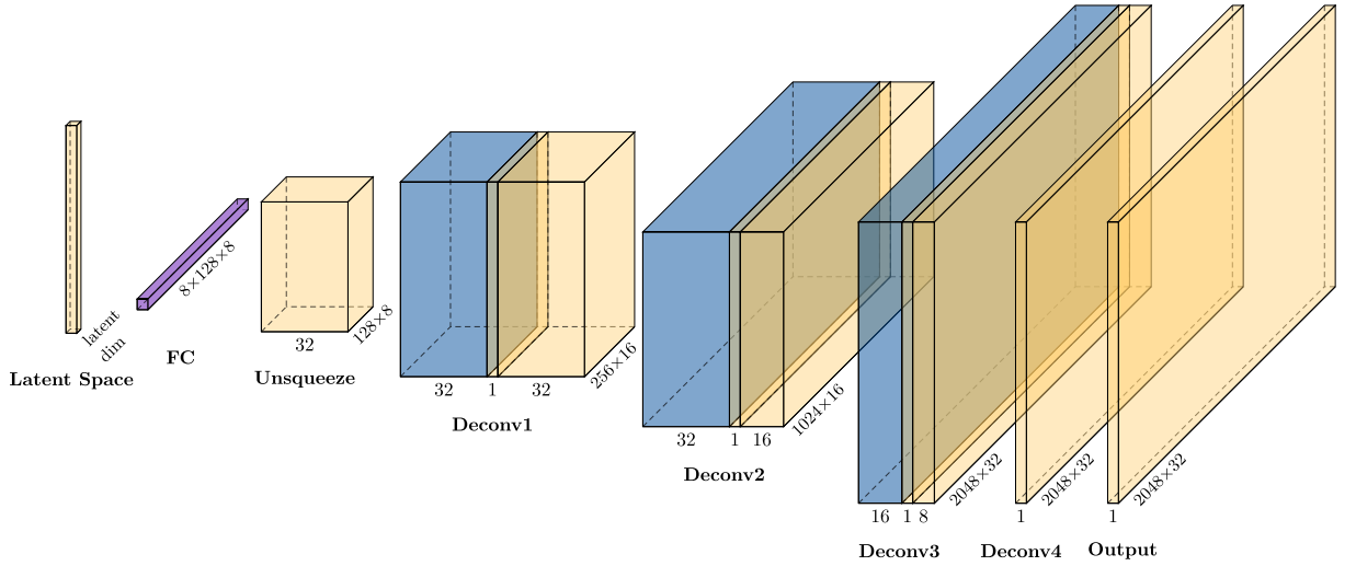
Figure 5.5: Architecture of the Efficient decoder. The input is a latent vector of dimension d . A fully connected layer first expands this into a feature map of size 8 \times 128 \times 8 , followed by a 1 \times 1 convolution ( Unsqueeze ) to increase the channel count to 32. The following three blocks ( Deconv1–3 ) each consist of nearest-neighbor upsampling and a depthwise-separable convolution: Deconv1 doubles both axes ( 32 \times 256 \times 16 ), Deconv2 restores horizontal resolution more aggressively with a 1 \times 4 upsampling ( 16 \times 1024 \times 16 ), and Deconv3 doubles both axes again to 8 \times 2048 \times 32 . The final block ( Deconv4 ) applies a (3 \times 17) convolution with circular padding along the azimuth, reducing the channels to 1 and producing the reconstructed output of size 1 \times 2048 \times 32 , which matches the original input dimensionality.
