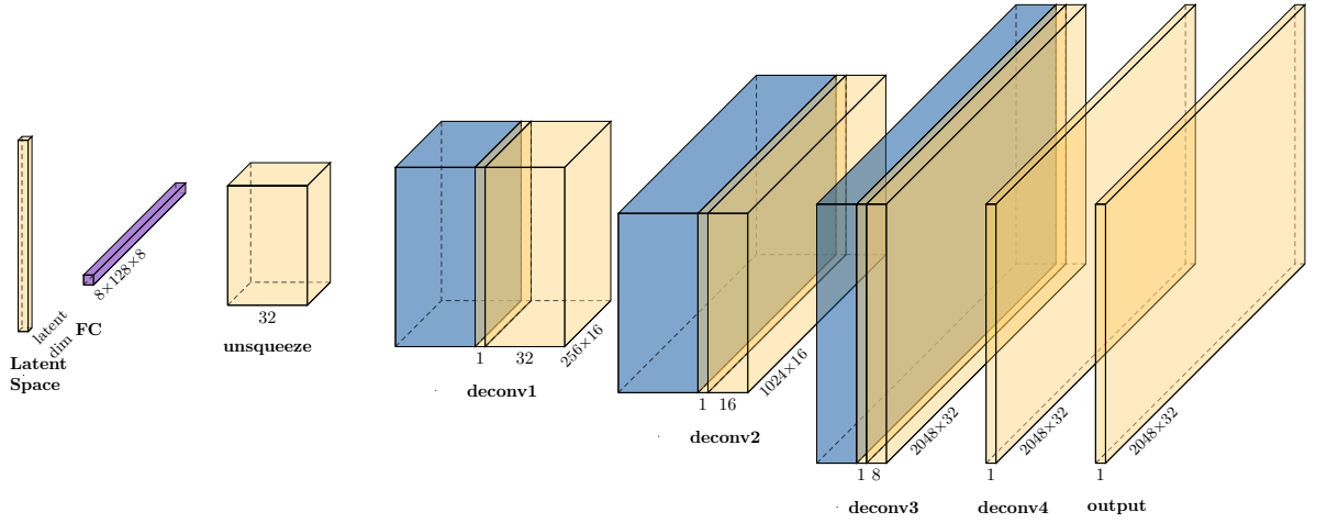
Figure 5.4: UNFINISHED - Visualization of the efficient decoder architecture.
