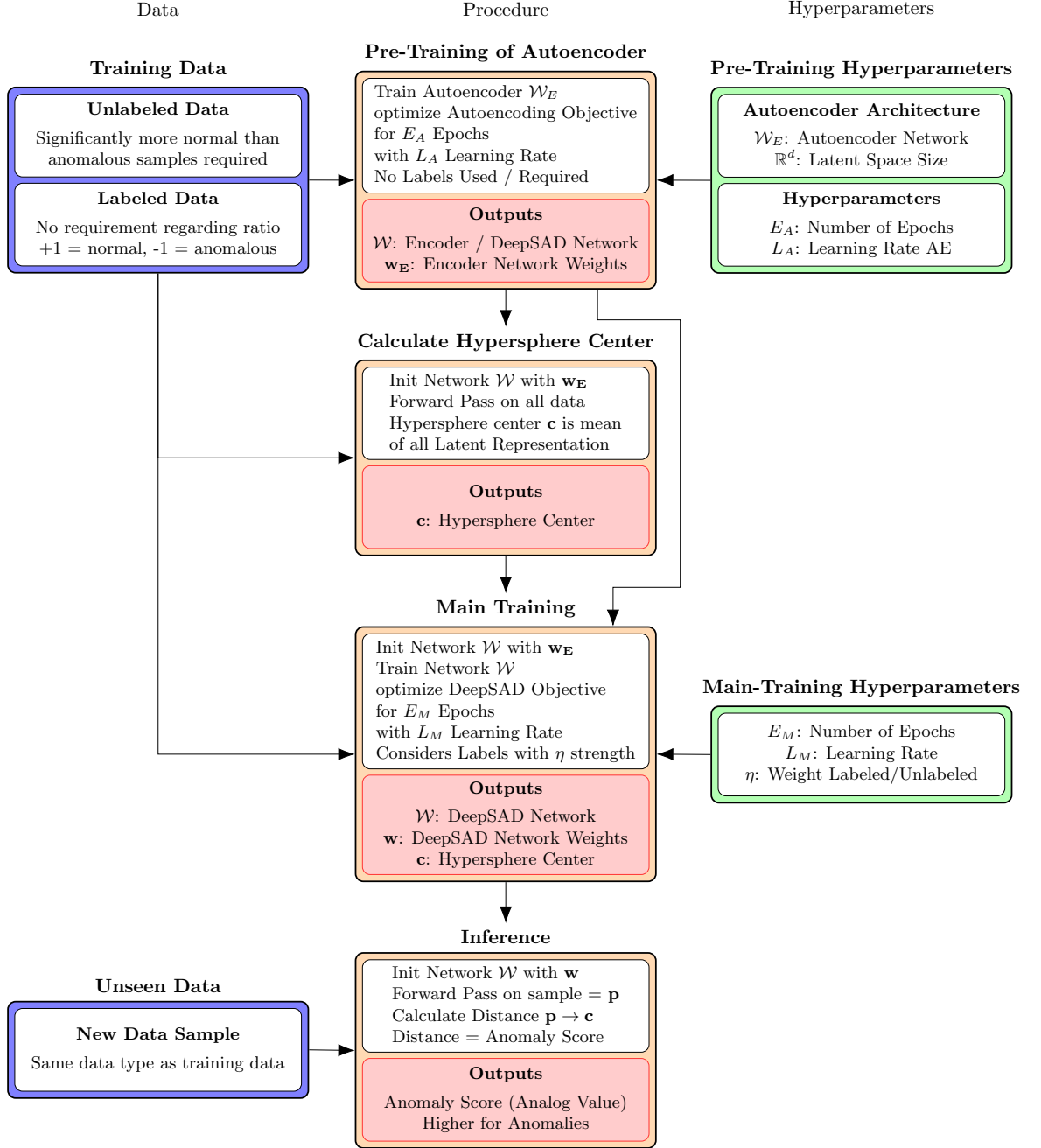
Figure 3.2: (WORK IN PROGRESS) Depiction of DeepSAD’s training procedure, including data flows and tweakable hyperparameters.
